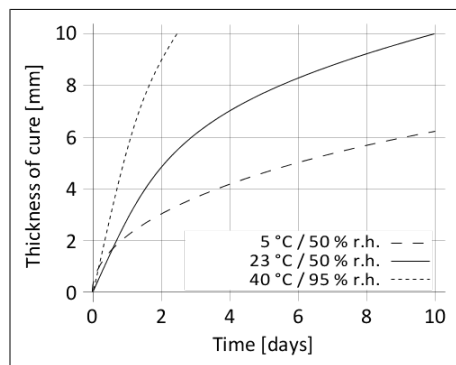
Diagram 1: Curing speed Sikasil® SG-20 S
